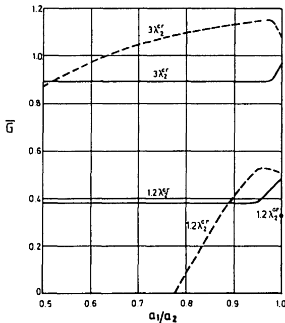
Fig. 6. Energy release rates, \bar{G} = G/E_1 t_1 \epsilon_0^2 , as a function of crack length ratio, a_1/a_2 , for a plate with two delaminations, E_1 = E_2 , \nu_1 = 0.35 , \nu_2 = 0.2 , t_1 = t_2 , \lambda_2 = 1.2\lambda_2^{cr} and \lambda_2 = 3\lambda_2^{cr} ; (---) lower crack 1, (—) upper crack 2 and (●) \bar{G}_1 at a_1 = a_2 .
