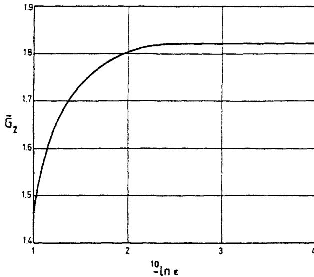
Fig. 13. Energy release rate, \bar{G}_2 = G_2/E_1 t_1 \epsilon_0^2 , as a function of the tolerance, \epsilon defined in (11), for a plate with two delaminations, E_1 = E_2 , \nu_1 = \nu_2 = 0.3 , a_1 = a_2 , t_2 = 1.5t_1 , \lambda_2 = 2\lambda_1^2 .
